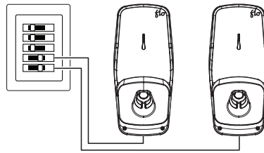
Dual circuit breaker setup
